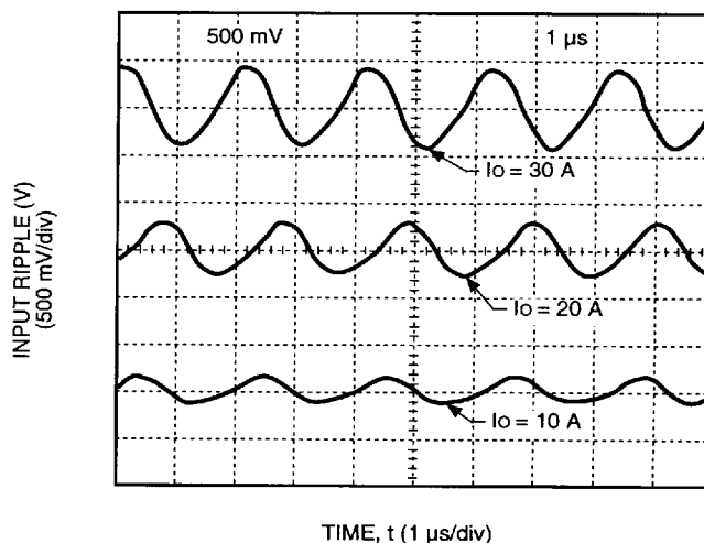
Figure 8. Typical FE150A Input Ripple Voltage at Room Temperature, 48 V Input, and 10 A, 20 A, and 30 A Output
