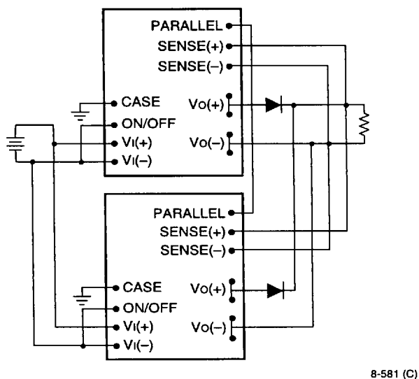
Figure 20. Wiring Configuration for Redundant Parallel Operation
