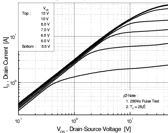
Fig 1. Output Characteristics
