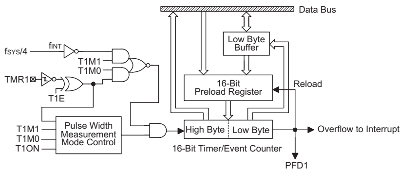
Timer/Event Counter 1
