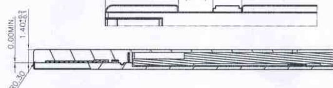
SEC B-B
