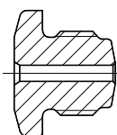
124452 DRIVING ANVIL -03
