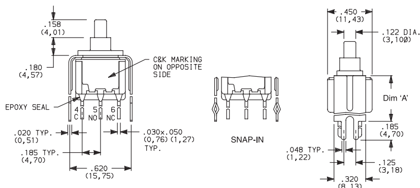
8221SD3_GE DPDT
