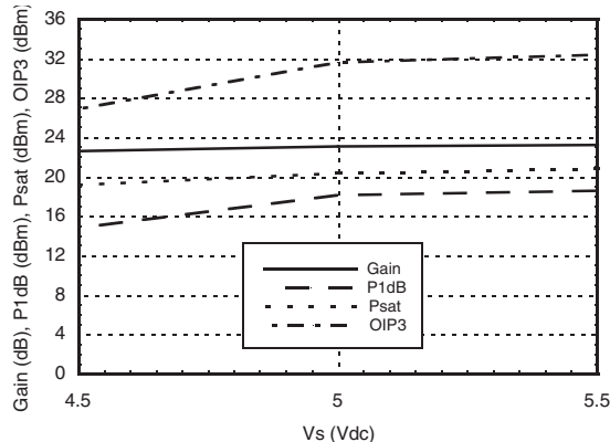
Gain, Power & OIP3 vs. Supply Voltage for Rs = 18 Ohms @ 850 MHz
