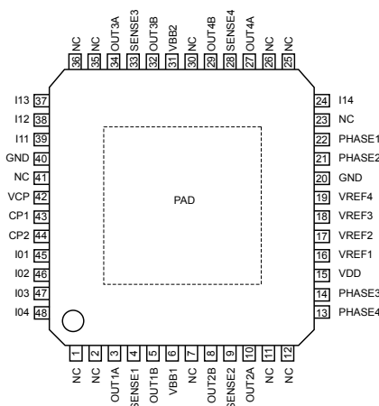
Package JP, 48-Pin LQFP Pin-out
