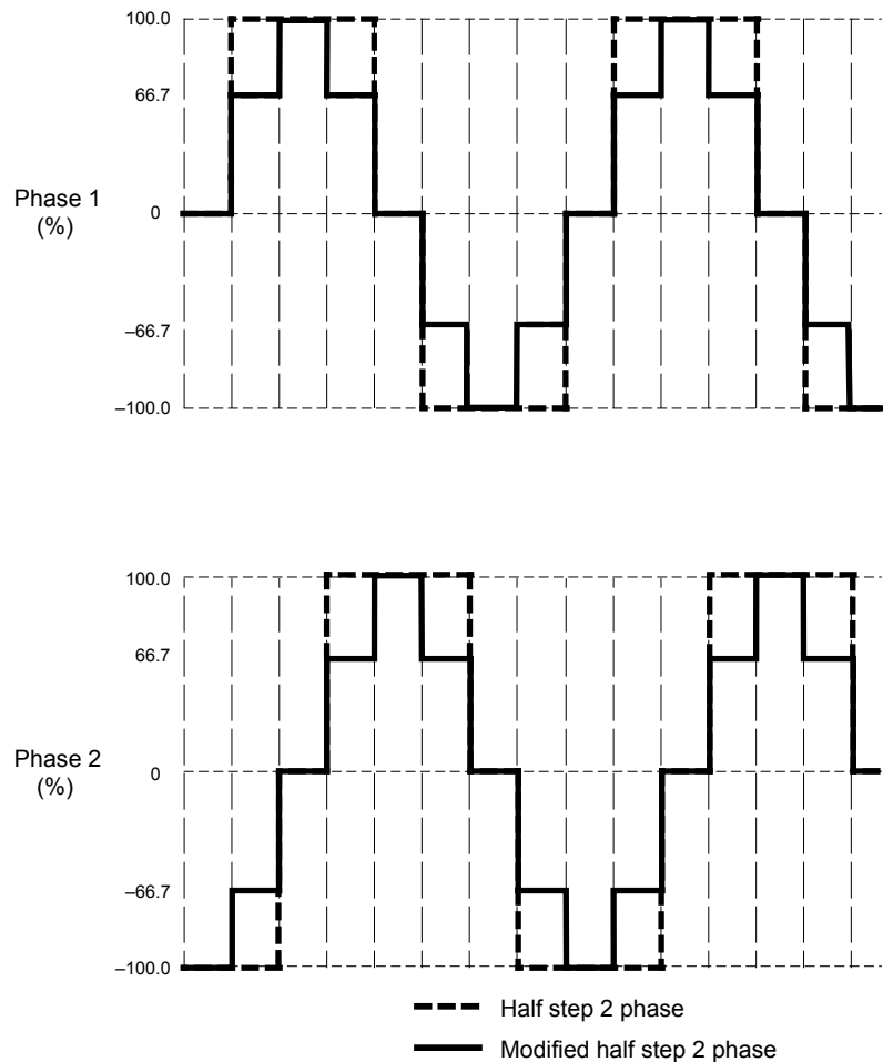
Figure 3: Step Sequencing for Half-Step Increments.
