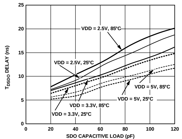
Figure 23. t_{DSDO} vs. Capacitance Load and Supply
