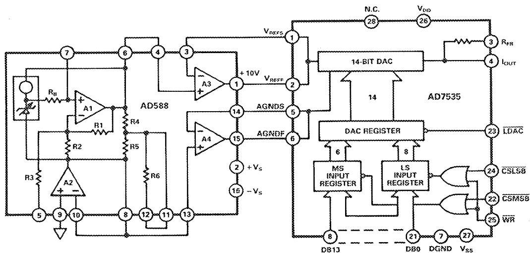
Figure 15. AD588/AD7535 Connections
