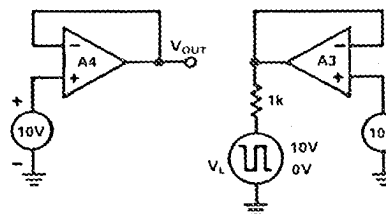
Figure 13a. Load Crosstalk Test Circuit
