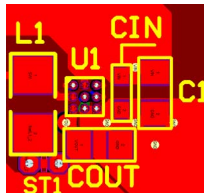
Figure 46. Fairchild Reference Board Layout
