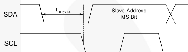
Figure 40. Start Bit
