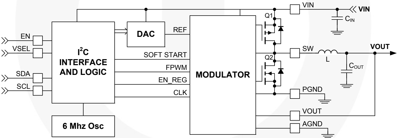
Figure 3 Block Diagram
