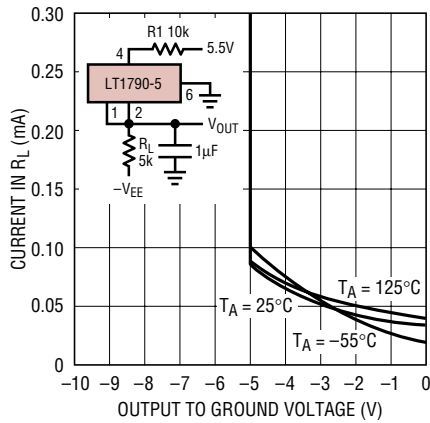
-5V Characteristics
