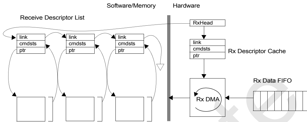
Figure 5-6 Receive Architecture
