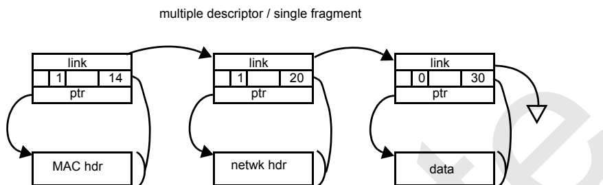
Figure 5-2 Multiple Descriptor Packets
