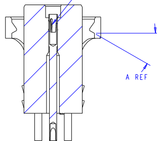
SECTION X-X
