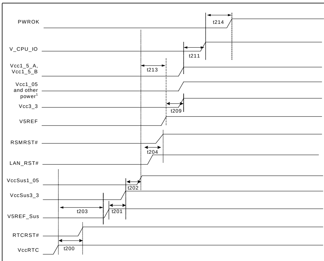
Figure 39. Power Sequencing and Reset Signal Timings
