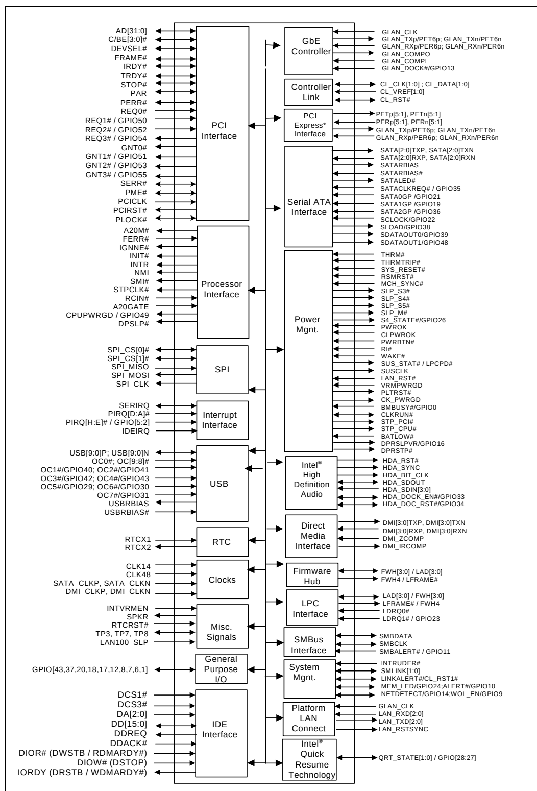
Figure 2. Intel® ICH8 Interface Signals Block Diagram (Mobile)
