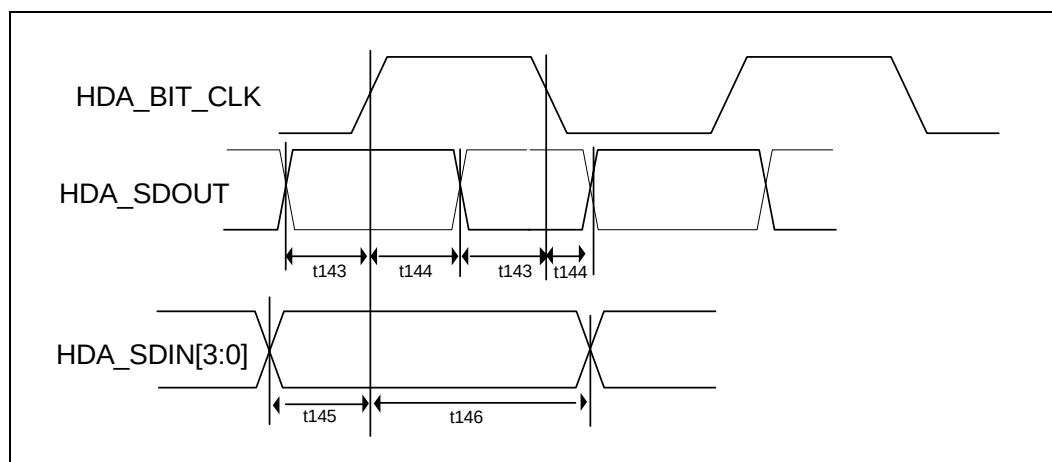
Figure 47. Intel® High Definition Audio Input and Output Timings
