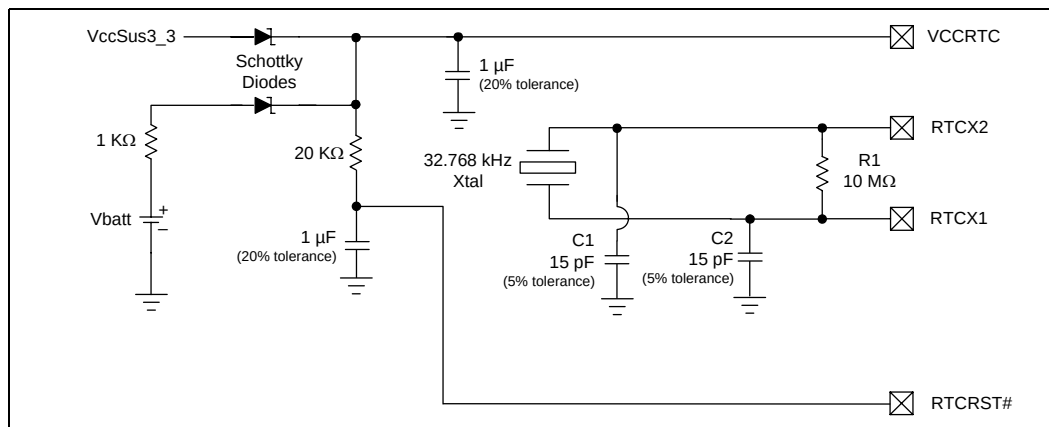
Figure 3. Example External RTC Circuit
