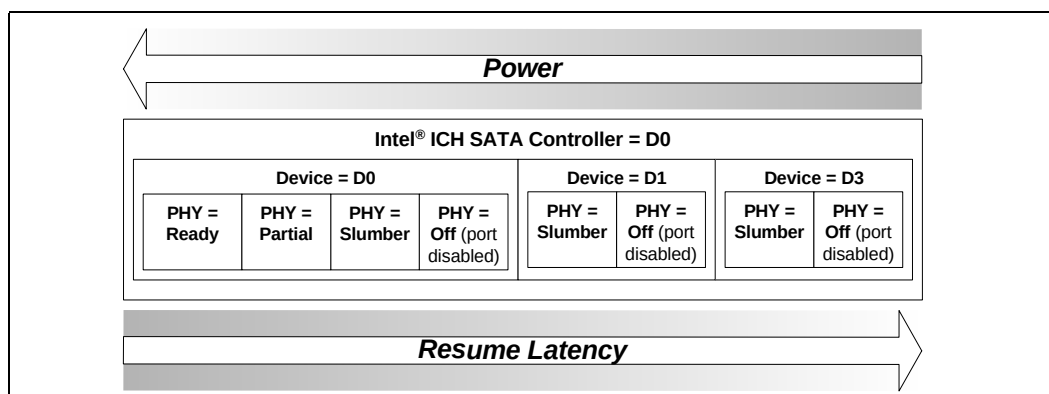
Figure 14. SATA Power States
