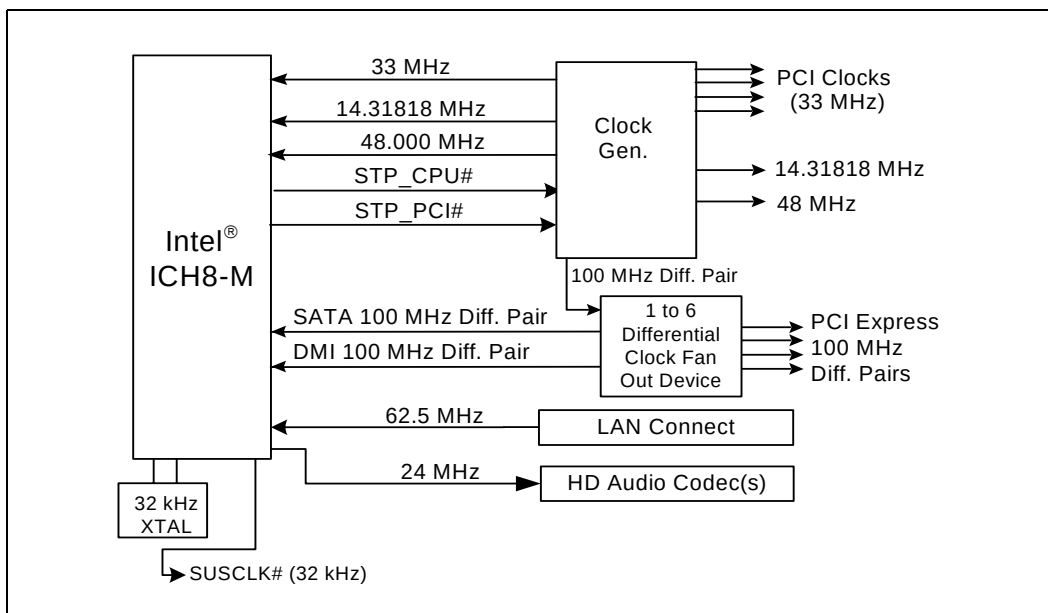
Figure 5. Mobile Conceptual Clock Diagram
