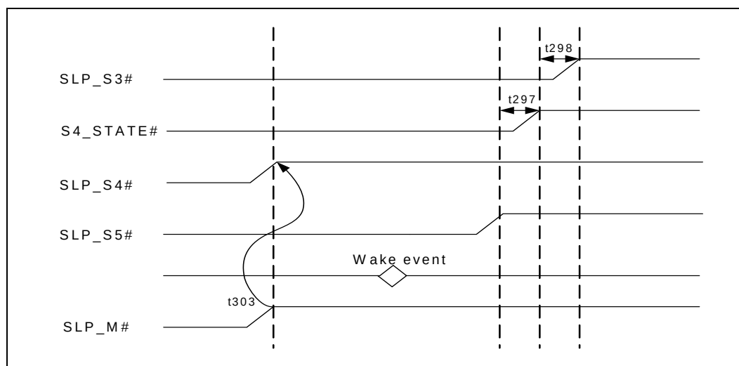
Figure 51. Sleep Control Signal Relationship – Host stays in S5 and ME boots after G3
