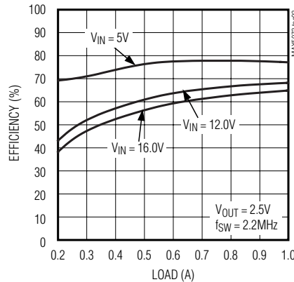
OUTPUT2 EFFICIENCY (BUCK CONVERTER) vs. LOAD CURRENT
