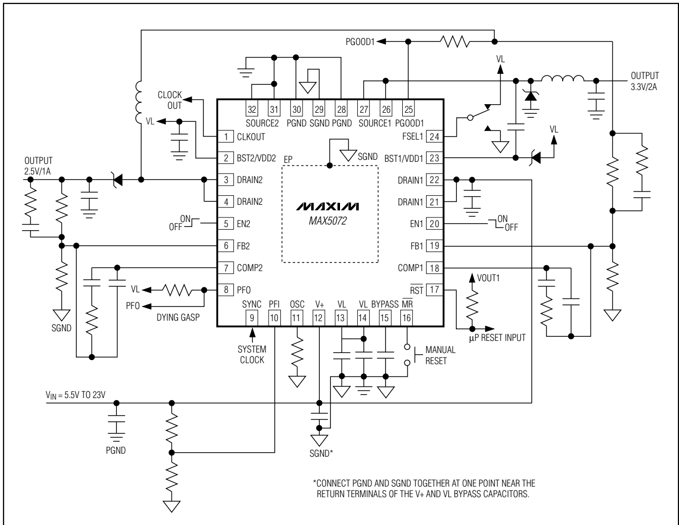
Figure 9. Buck-Boost Application
