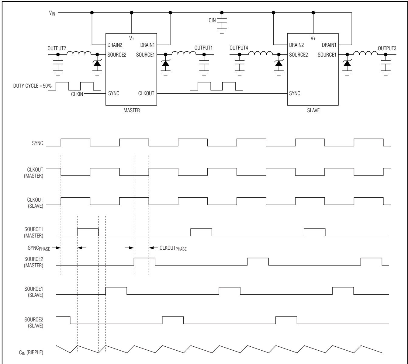
Figure 3. Synchronized Controllers
