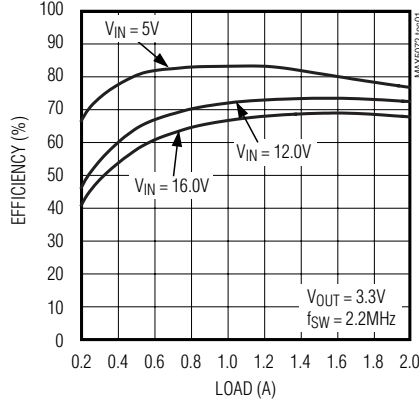
OUTPUT1 EFFICIENCY (BUCK CONVERTER) vs. LOAD CURRENT
