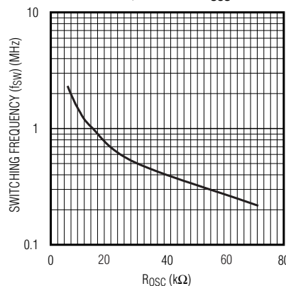
EACH CONVERTER SWITCHING FREQUENCY vs. R0SC
