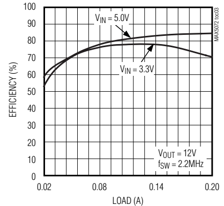
OUTPUT2 EFFICIENCY (BOOST CONVERTER) vs. LOAD CURRENT
