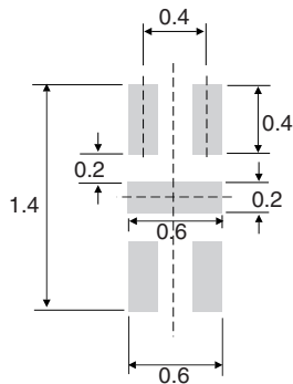
Figure 11. Footprint recommendations (dimensions in mm)
