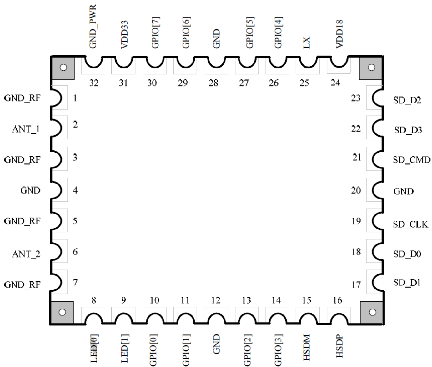
Figure 2: Module Pinout
