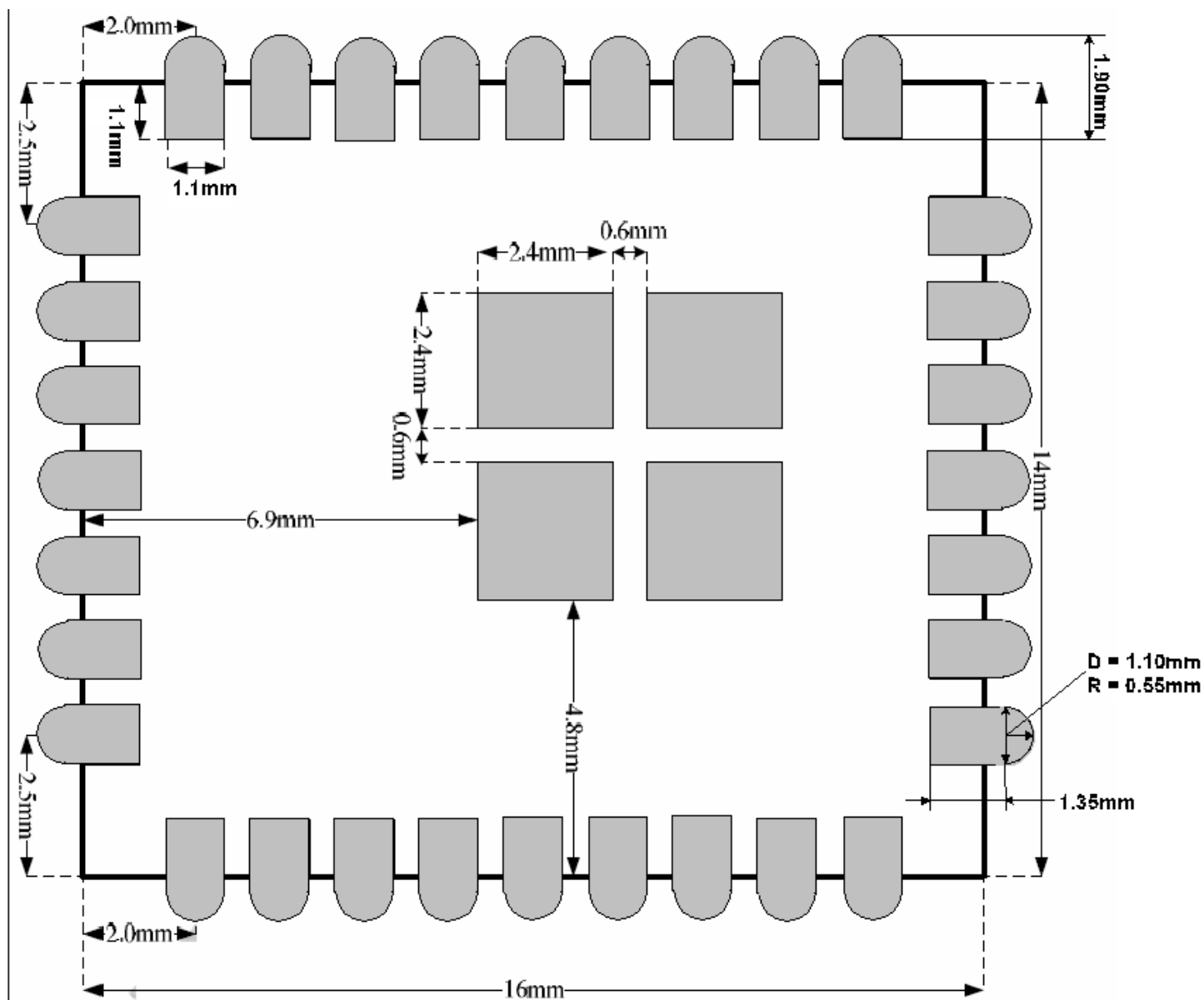
Figure 6: Mechanical Drawing 2
