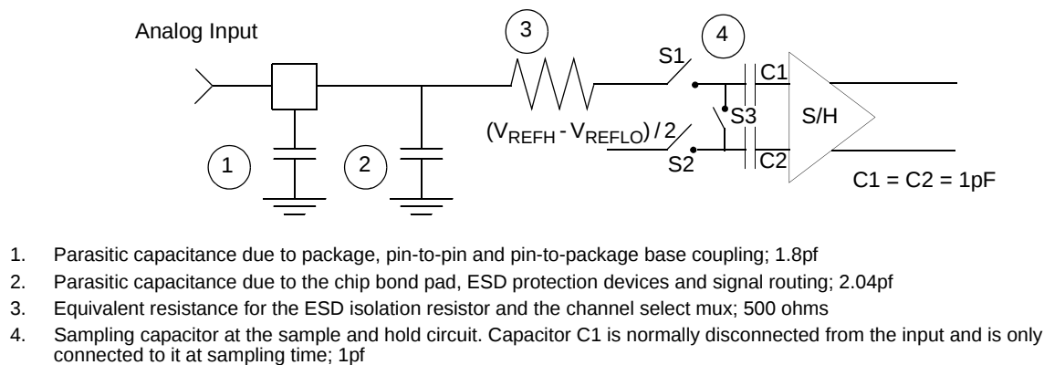
Figure 10-22 Equivalent Circuit for A/D Loading
