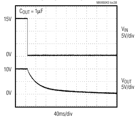
TURN-OFF TRANSIENT
