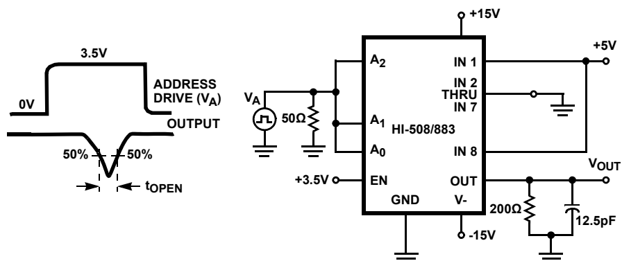
BREAK-BEFORE-MAKE DELAY ( t_{\text{OPEN}} )
