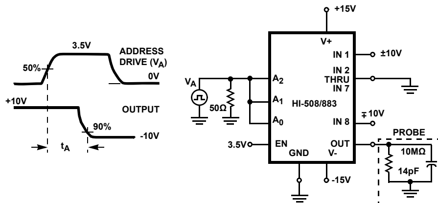
ACCESS TIME vs LOGIC LEVEL (HIGH)
