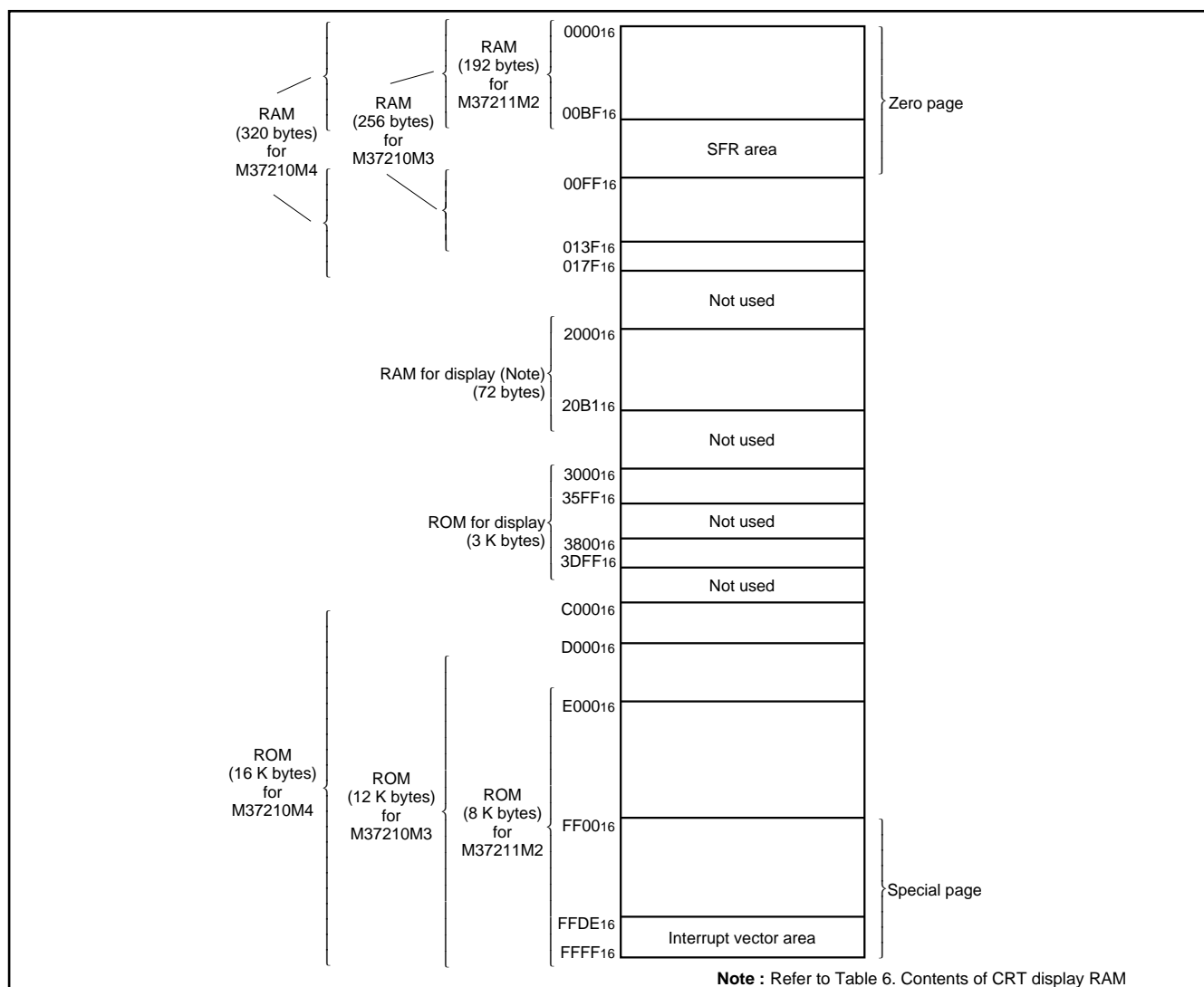
Fig. 2 Memory map
