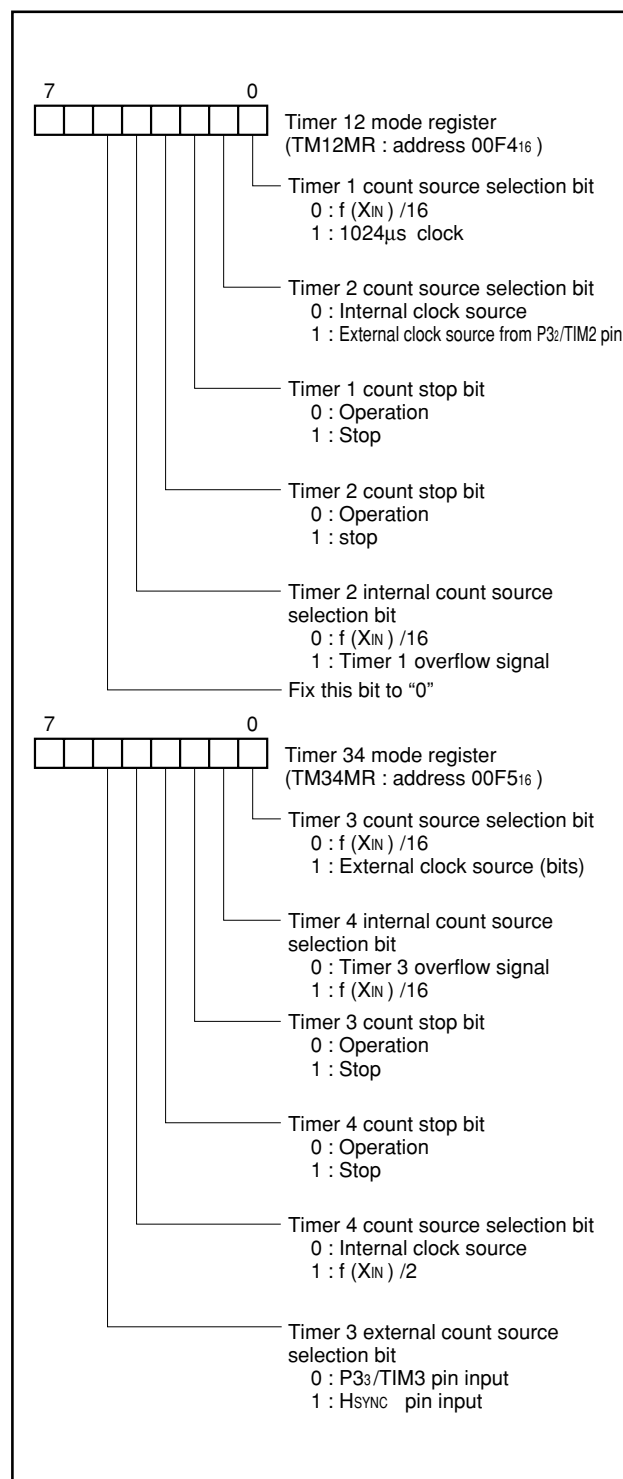
Fig. 6 Structure of timer-related registers
