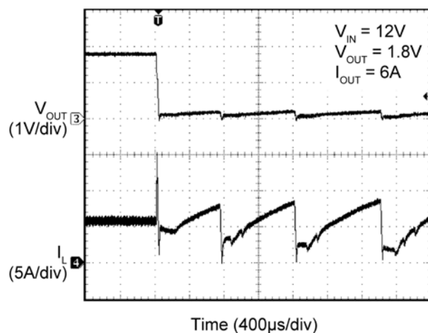
Short Circuit
