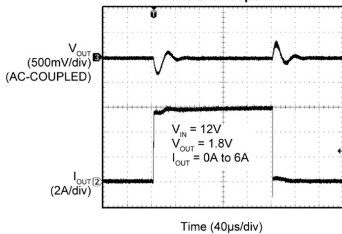
Transient Response
