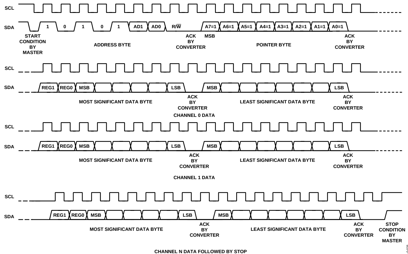
Figure 35. 2-Byte Mode I²C Write Operation
