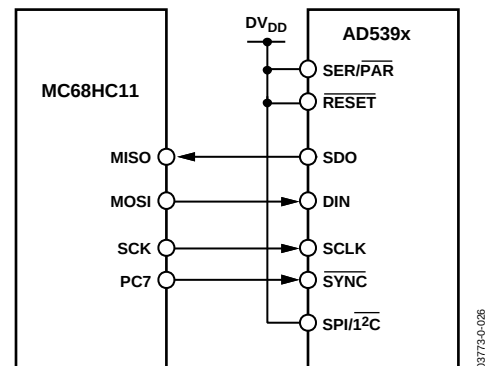
Figure 36. AD539x-MC68HC11 Interface
