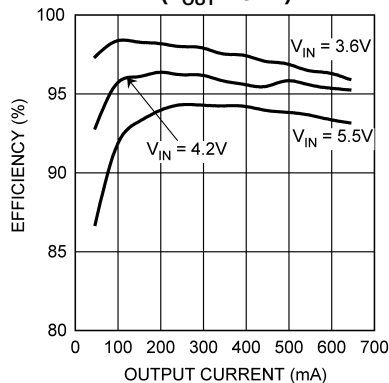
Efficiency vs Output Current ( V_{OUT} = 3.4V )
