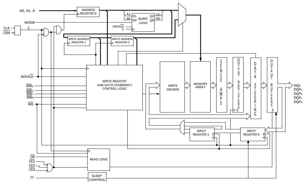
Logic Block Diagram—CY7C1370CV25 (512K x 36)
