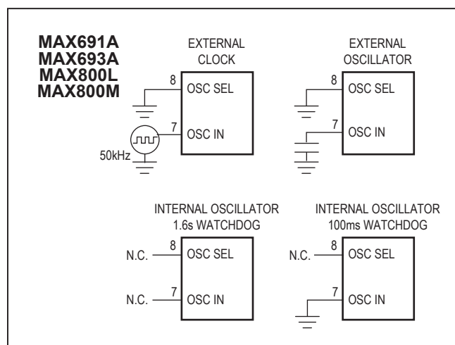
Figure 3. Oscillator Circuits
