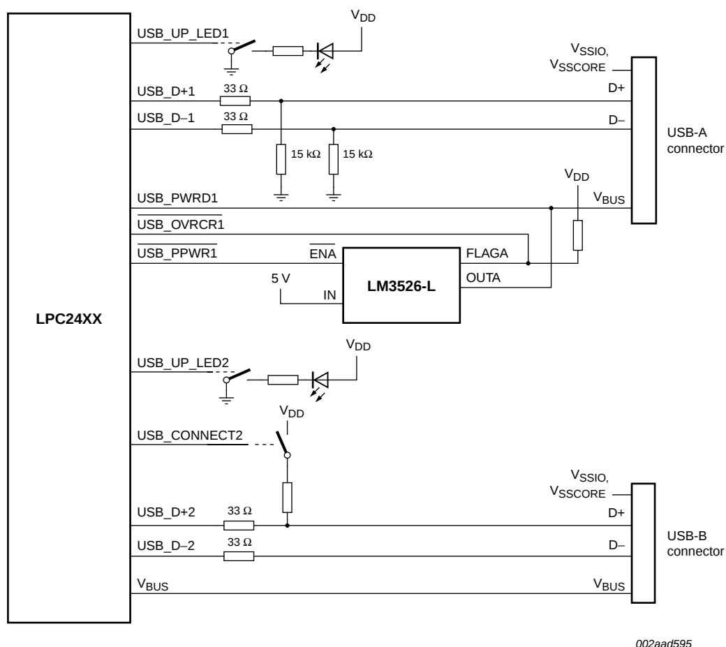
Fig 27. LPC2470 USB OTG port configuration: USB port 2 device, USB port 1 host
