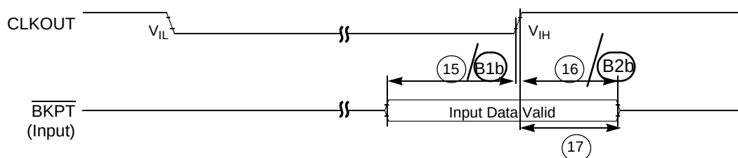
Figure 33-20. \overline{\text{BKPT}} Timing
