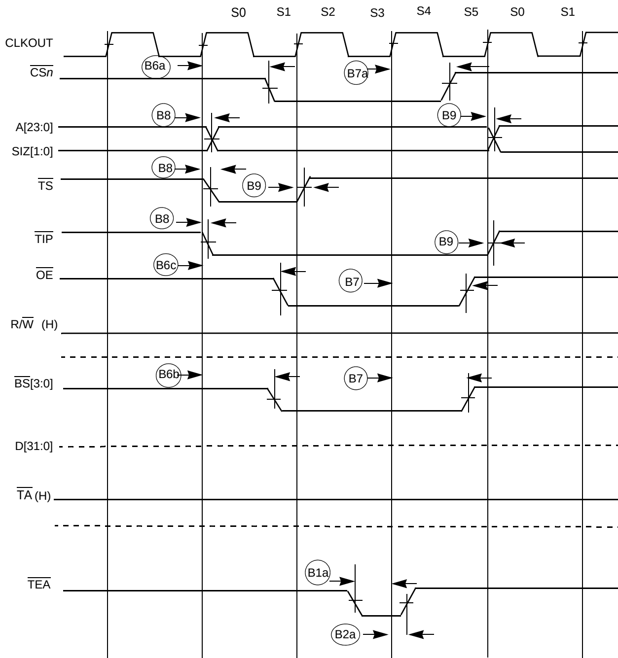
Figure 33-5. Read Bus Cycle Terminated by \overline{\text{TEA}}
