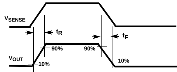
FIGURE 12. OUTPUT CURRENT RISE AND FALL TIME
