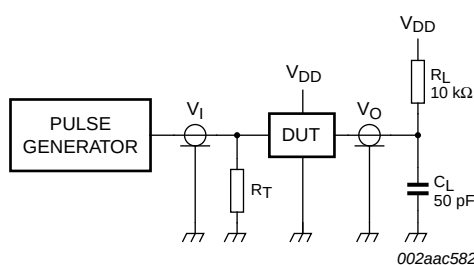
Fig 18. Test circuitry for switching times, \overline{INT}
