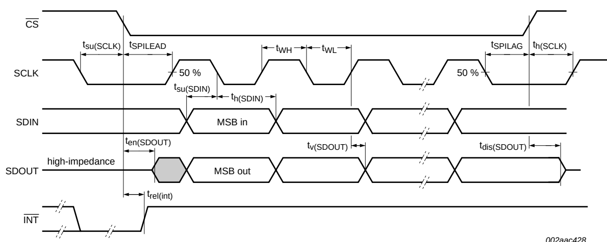
Fig 13. Timing diagram
