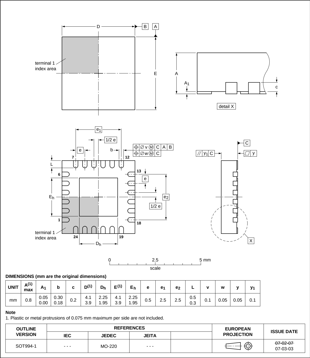
Fig 20. Package outline SOT994-1 (HWQFN24)
