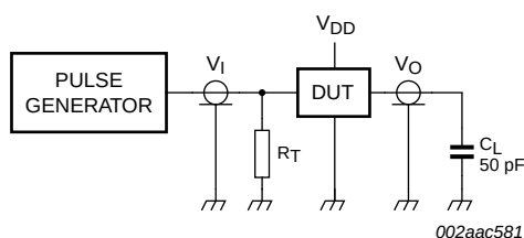
Fig 17. Test circuitry for switching times, SDOUT ( t_v(SDOUT) )
