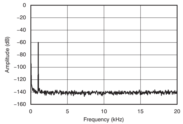
Figure 17. Output Spectrum
