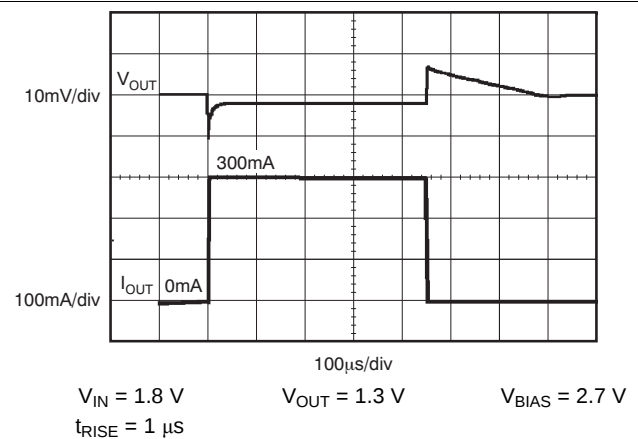
Figure 26. Load Transient Response
