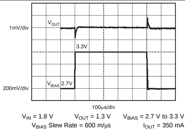
Figure 25. V_{\text{BIAS}} Line Transient Response
