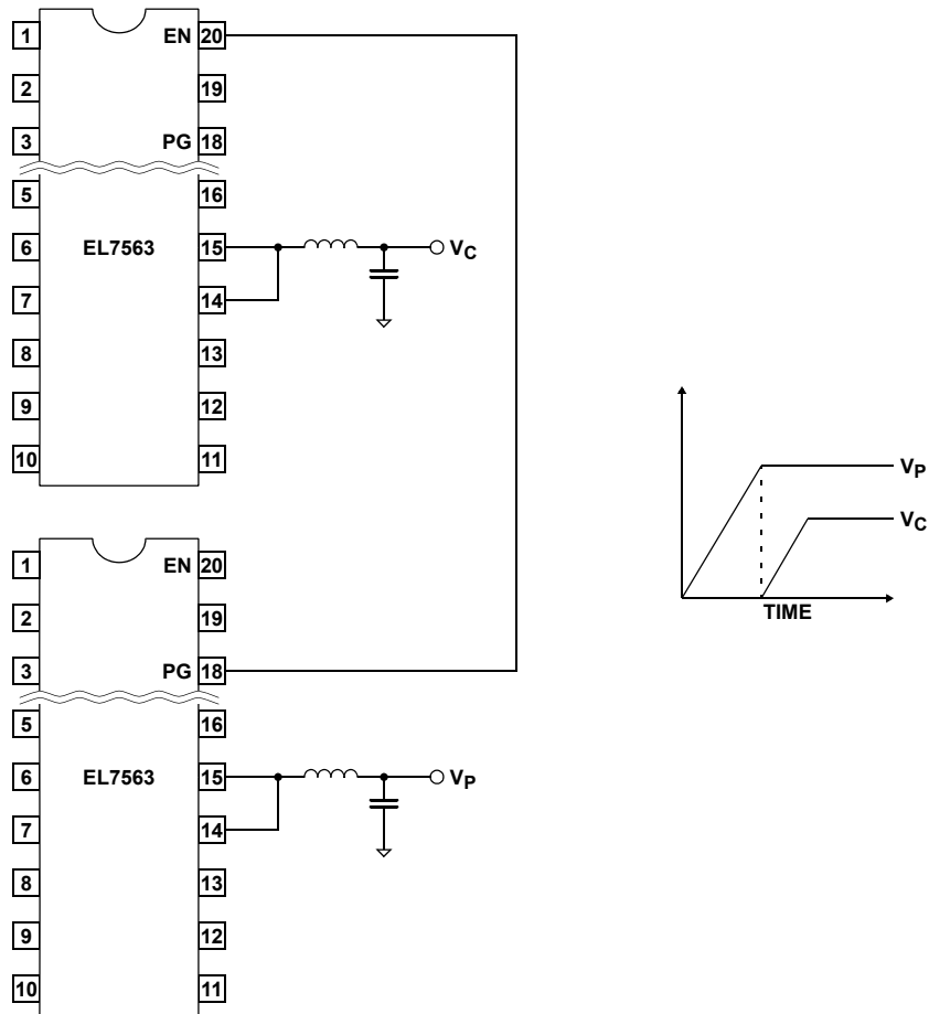
FIGURE 25. OFFSET TRACKING
