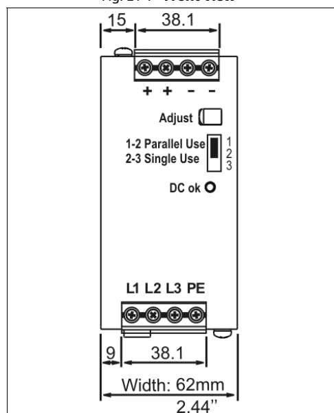
Fig. 21-1 Front view
