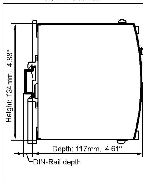
Fig. 21-2 Side view
