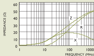
PBY201209T-300Y-S
