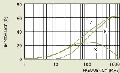
PBY160808T-400Y-S
