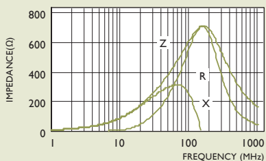
PBY160808T-601Y-S
