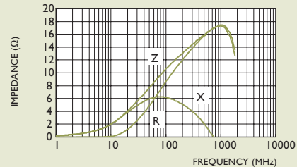
PBY100505T-100Y-S
