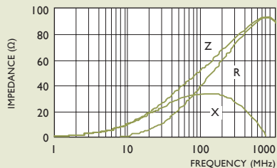
PBY160808T-600Y-S
