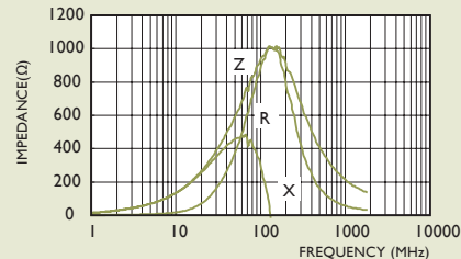
PBY160808T-102Y-S
