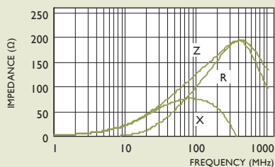
PBY160808T-121Y-S
