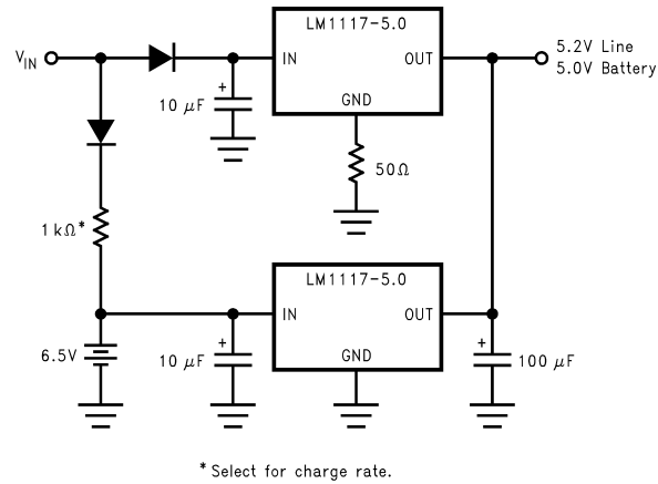
Figure 37. Battery Backed-Up Regulated Supply
