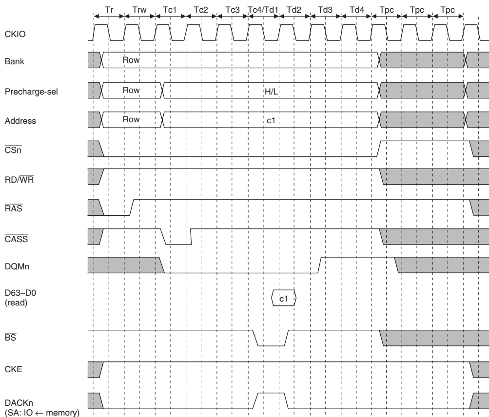
Figure 13.29 Basic Timing for Synchronous DRAM Single Read
