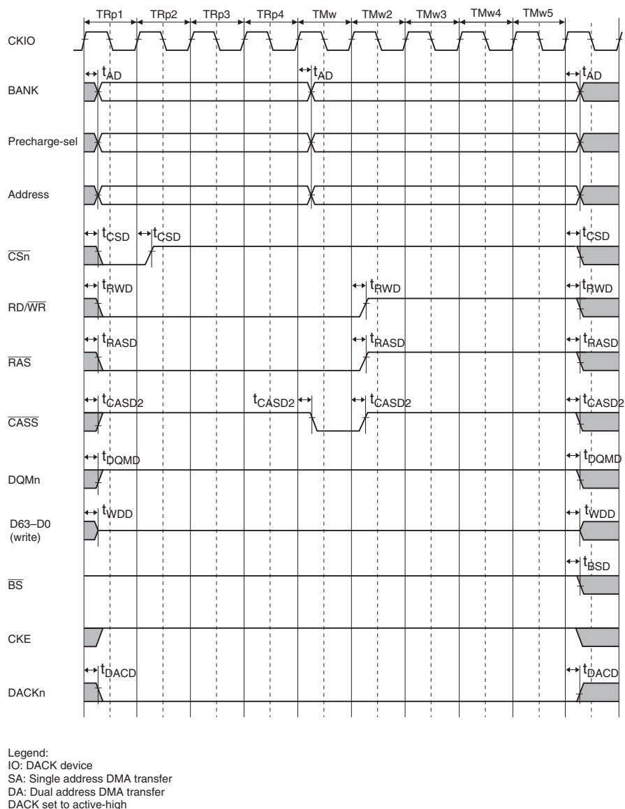
Figure 22.36 (a) Synchronous DRAM Bus Cycle: Synchronous DRAM Mode Register Setting (PALL)
