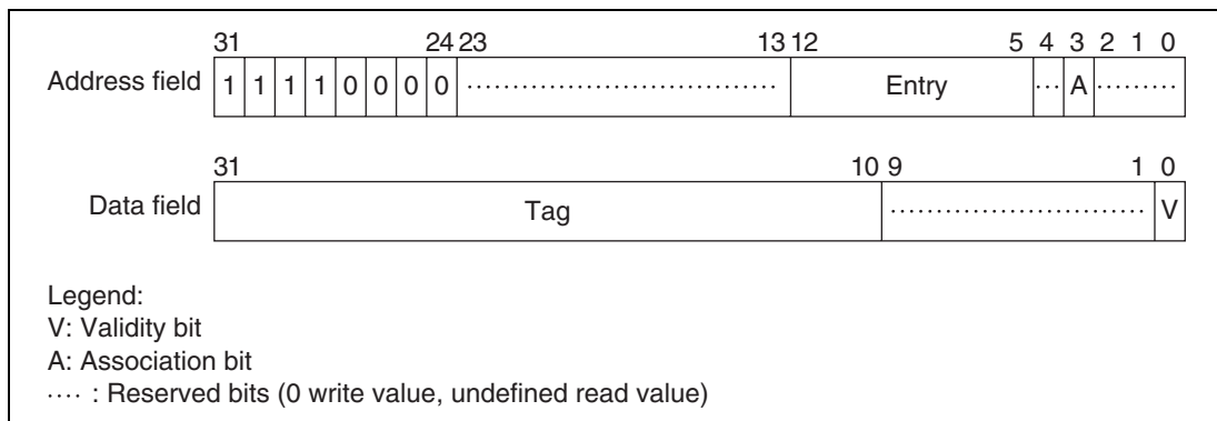
Figure 4.8 Memory-Mapped IC Address Array
