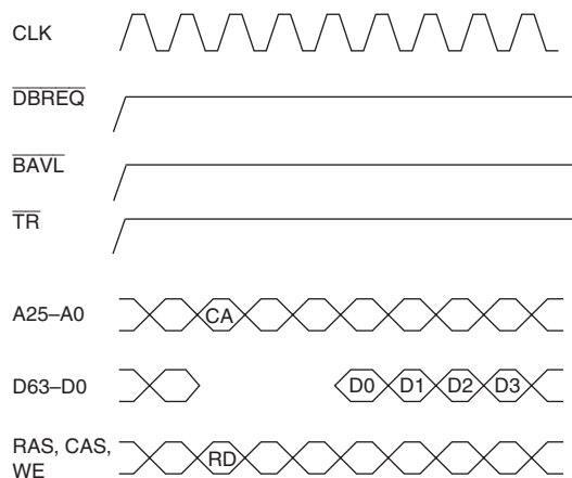
Figure 14.37 Read from Synchronous DRAM (Row Hit)
