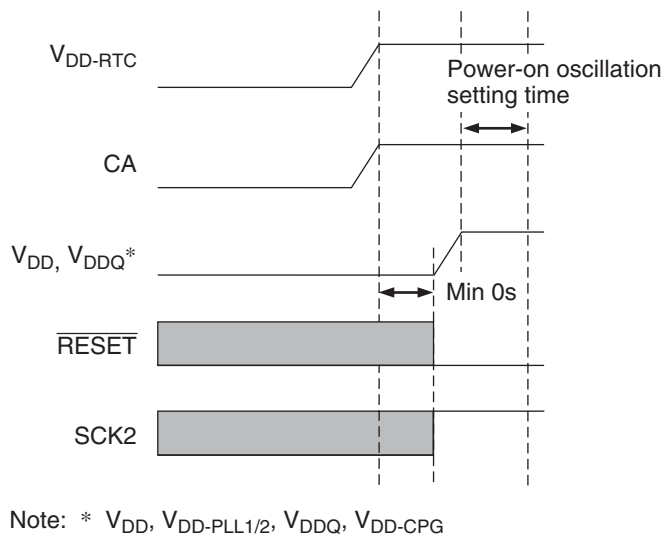
Figure 9.15 Timing When VDD-RTC Power Is Off → On
