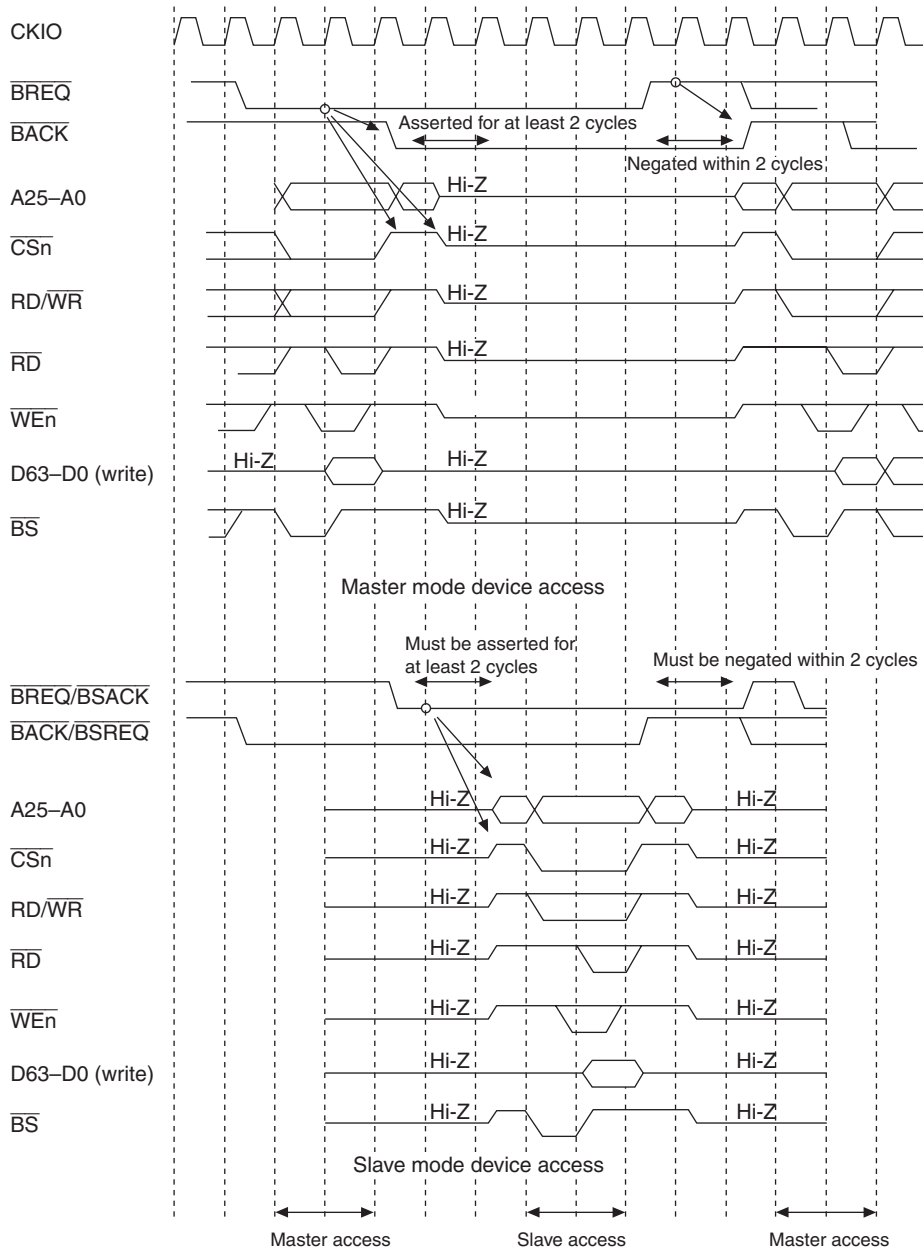
Figure 13.79 Arbitration Sequence
