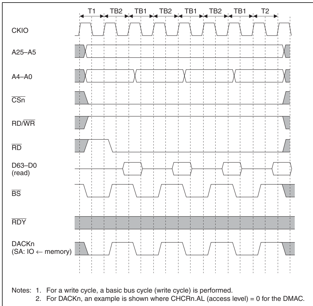
Figure 13.47 Burst ROM Basic Access Timing
