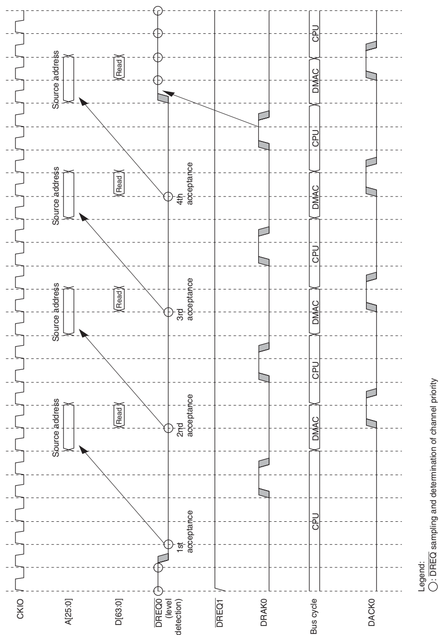
Figure 14.18 Single Address Mode/Cycle Steal Mode External Bus → External Bus/DREQ (Level Detection)
