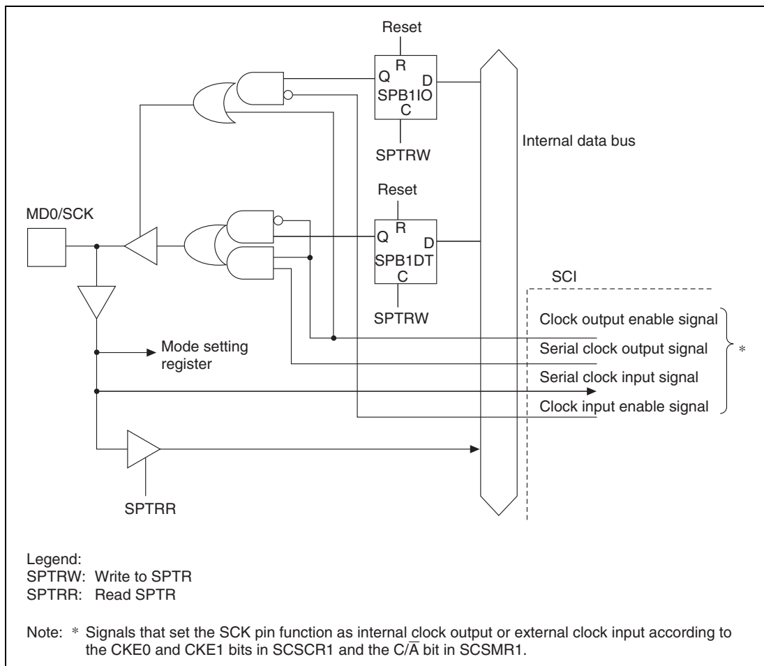
Figure 18.3 MD0/SCK Pin
