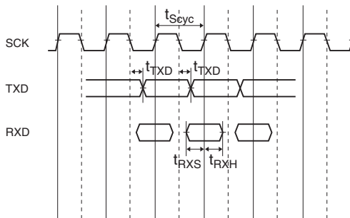
Figure 22.64 SCI I/O Synchronous Mode Clock Timing
