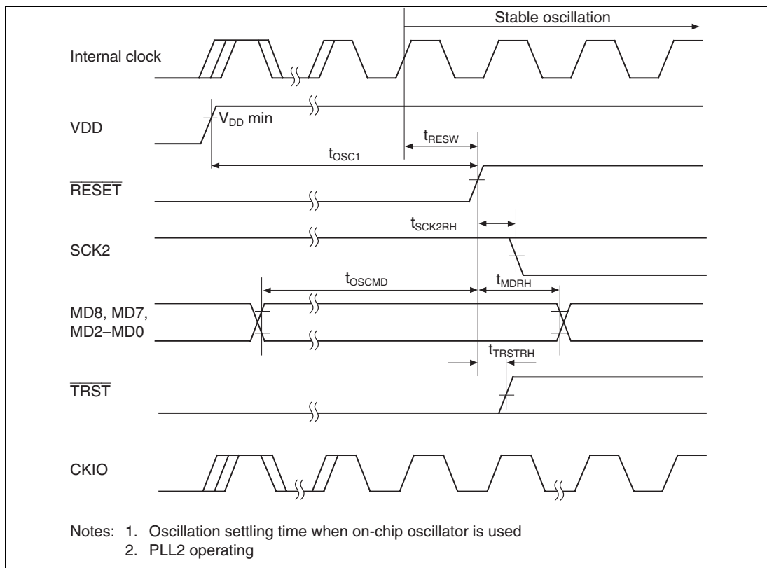
Figure 22.5 Power-On Oscillation Settling Time
