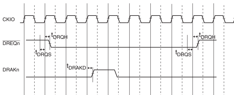
Figure 22.66 (a) \overline{\text{DREQ}} /DRAK Timing
