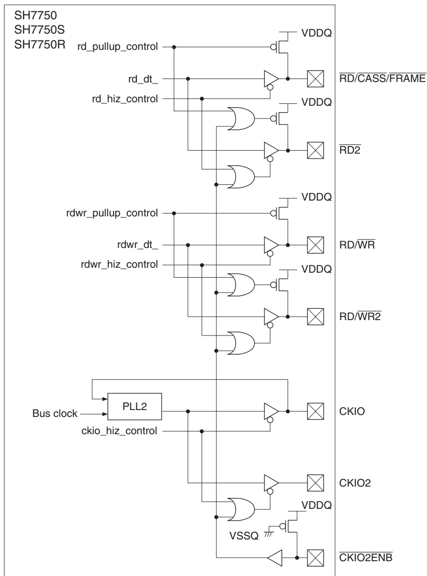
Figure D.1 CKIO2ENB Pin Configuration
