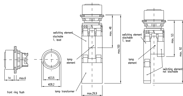
24 Illuminated pushbutton actuator page 17
