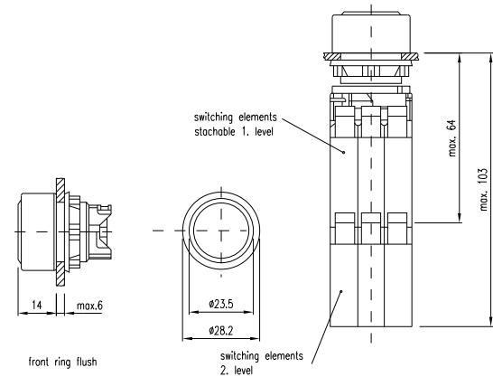
24 Illuminated pushbutton actuator page 17
