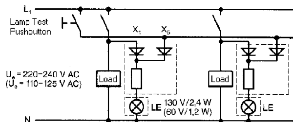
Diode resistance element
