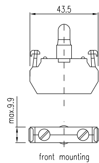
41 Slow-make switching element non-stackable, base mounting page 43
