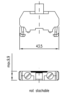
42 Lamp transformer page 46
