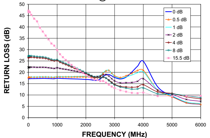
RETURN LOSS OUT (Major Atten. Steps) @ +25°C
