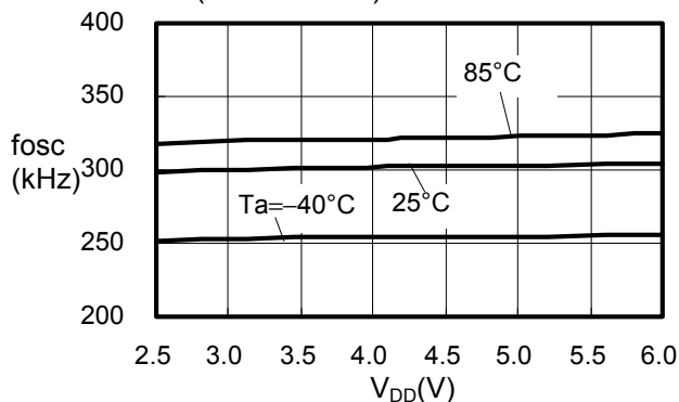
S-8340C33A(fosc:300 kHz)
