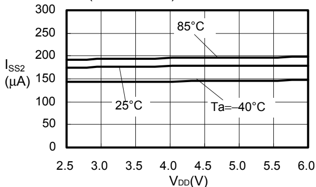
S-8340A33A(fosc:600 kHz)
