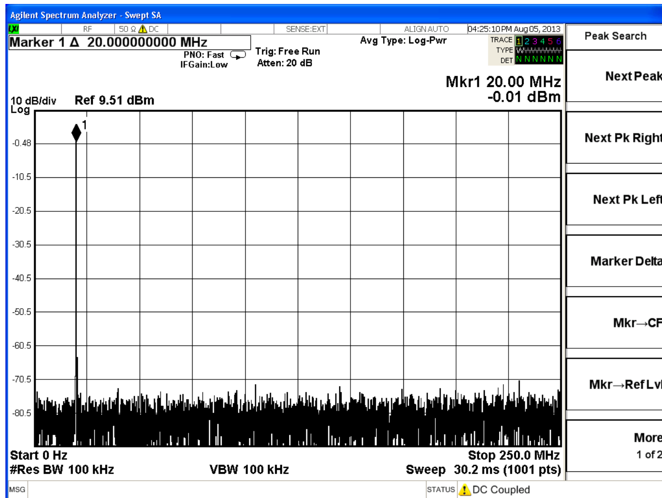
Figure 3. Spectrum with CLK2 = 500 MHz, X4L Interpolation and NCO Frequency = 343597383
