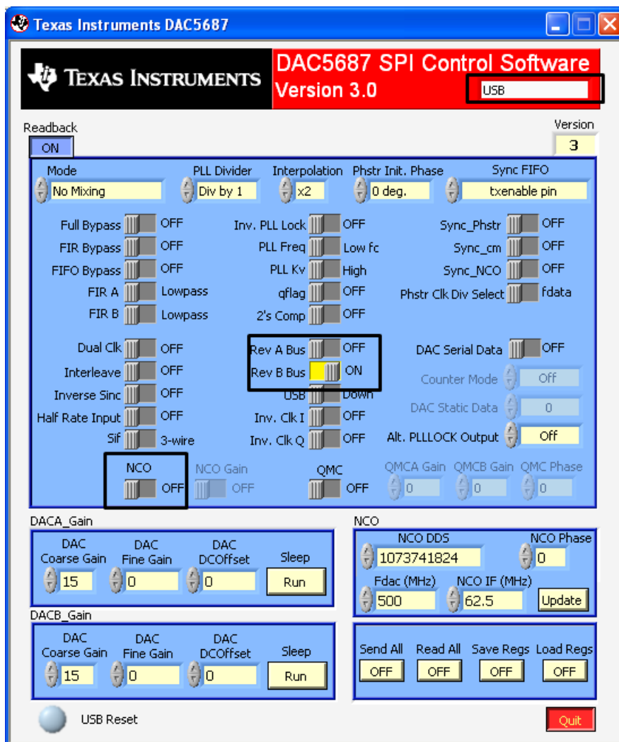
Figure 7. DAC5687 GUI Setup
