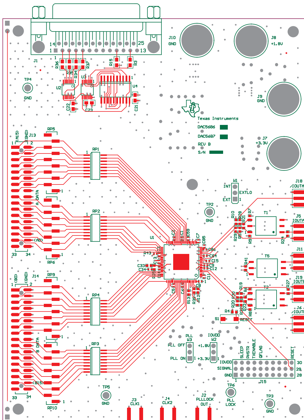
Figure 14. Top Layer 1
