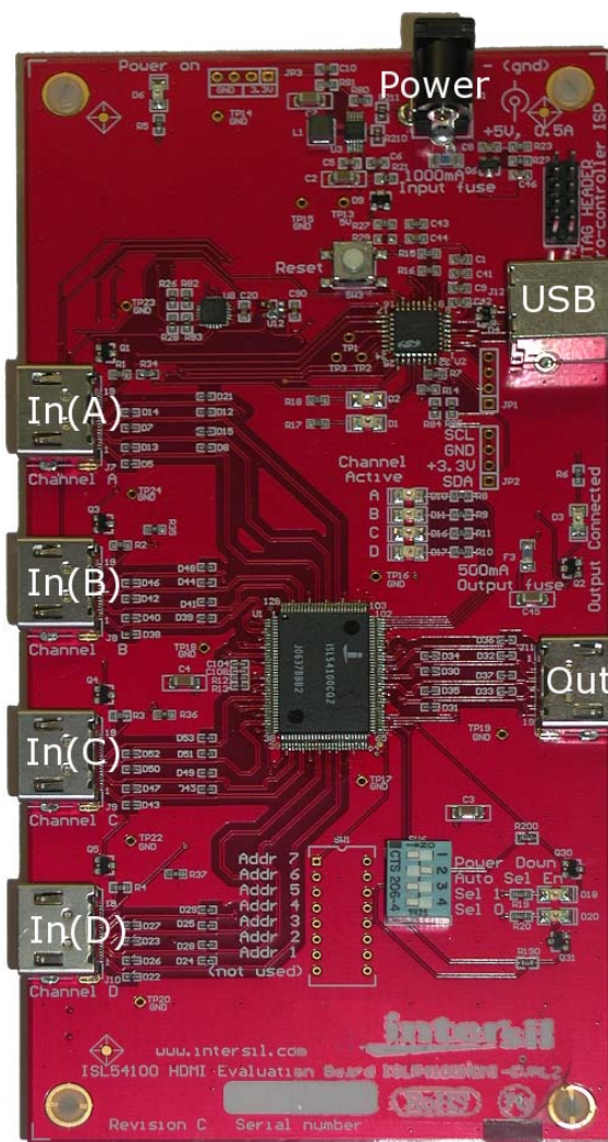
FIGURE 10. ISL54100AHDMI-EVALZ BOARD WITH PORT LABEL
