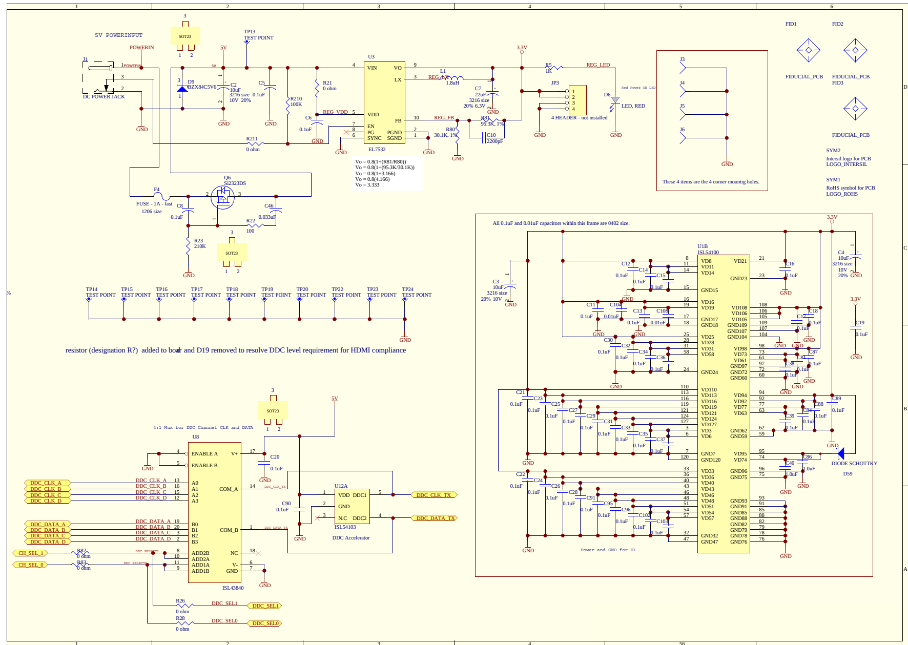
FIGURE 24. ISL54100AHDMI-EVALZ POWER/DDC
