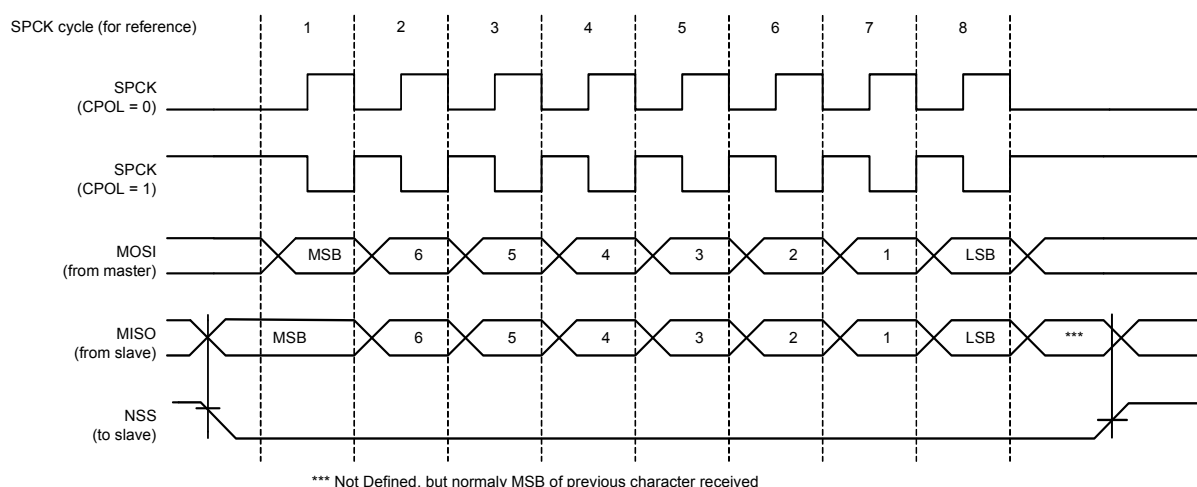
Figure 21-3. SPI Transfer Format (NCPHA = 1, 8 bits per transfer)
