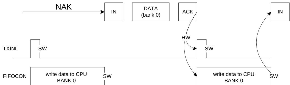
Figure 27-16. Example of an IN Endpoint with 1 Data Bank
