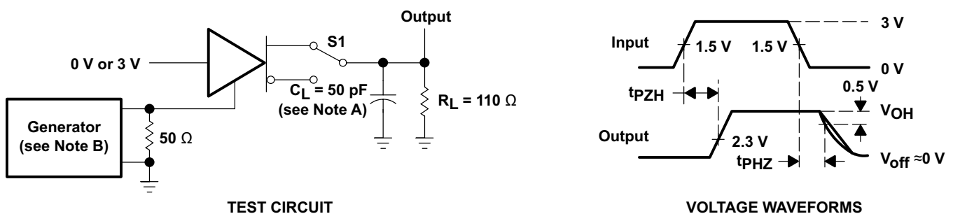
Figure 12. Driver Test Circuit and Voltage Waveforms
