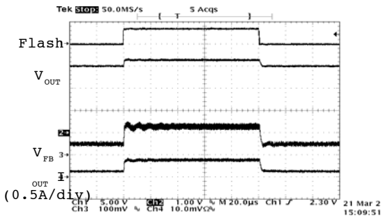
Figure 17. Torch in 1X to Flash 1X Mode, V_{in}=4.2\text{V} , C_{in}=4.7\mu\text{F} , C_{FC}=0.47\mu\text{F} , C_{out}=2.2\mu\text{F}
