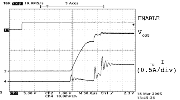
Figure 16. Startup Flash, V_{in}=3.6\text{V} , V_{out}=3.5\text{V} C_{in}=4.7\mu\text{F} , C_{FC}=0.4\mu\text{F} , C_{out}=2\mu\text{F}
