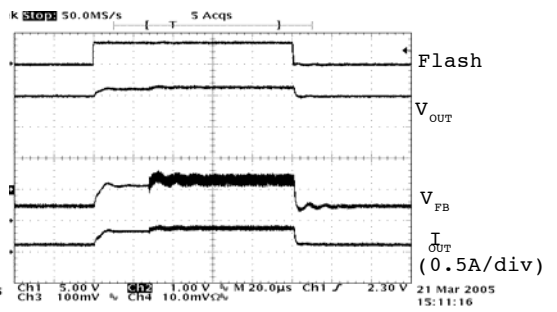
Figure 18. Torch in 1X to Flash 2X Mode, V_{in}=3.6\text{V} , C_{in}=4.7\mu\text{F} , C_{FC}=0.47\mu\text{F} , C_{out}=2.2\mu\text{F}
