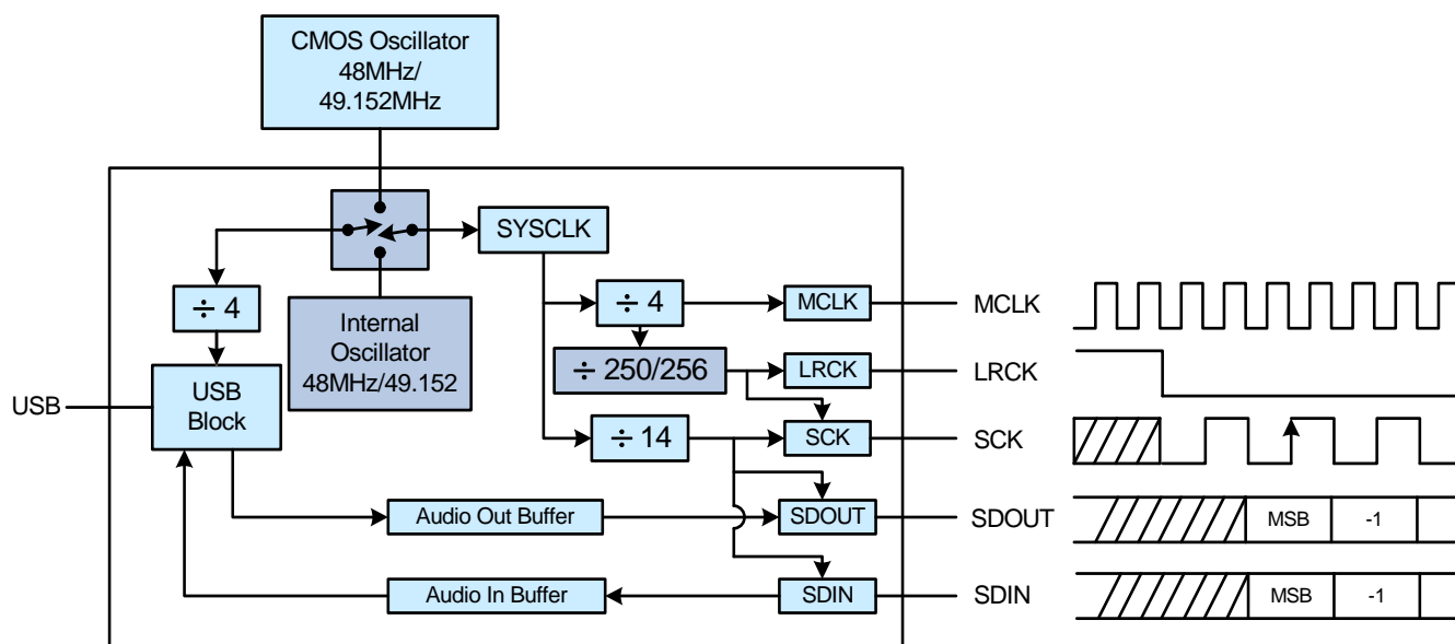
Figure 10. Clock Configuration Block Diagram
