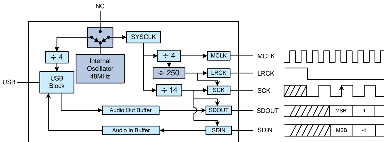
Figure 11. Configuration 1 Example
