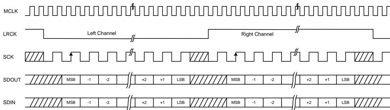
Figure 8. I2S Format
