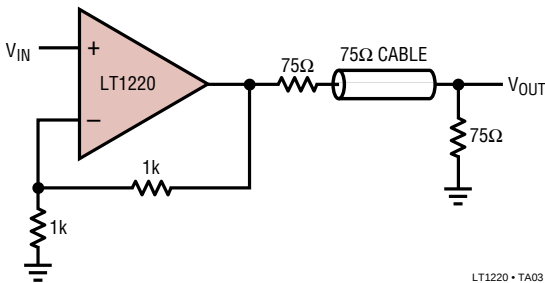
Cable Driver
