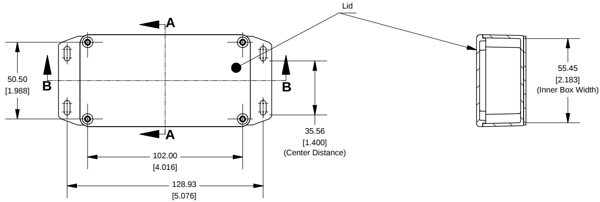
SECTION A-A End View of Assembly
