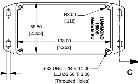
Top View Looking Inside Box C
