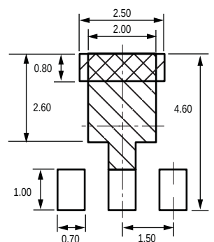
PCB Layout Reference View
